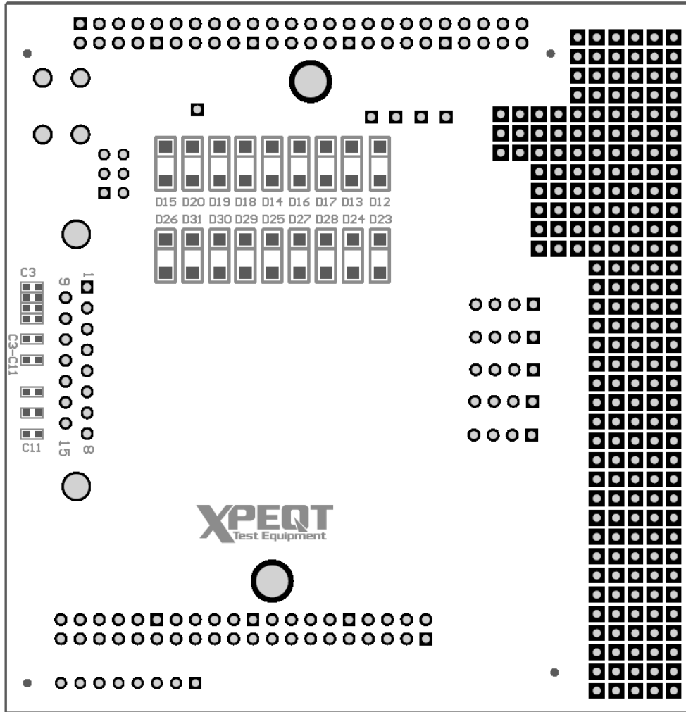
Figure 3: Board Layout Bottom Layer.
