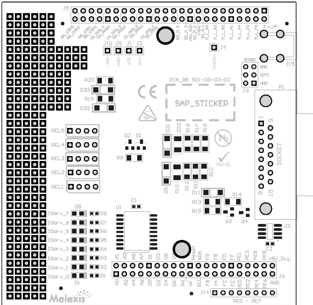
Figure 2: Board Layout Top Layer.
