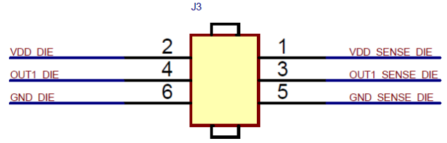
Figure 6: Jumper between force and sense line.
