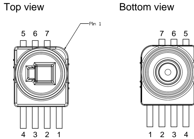
Figure 3: Package pinout
