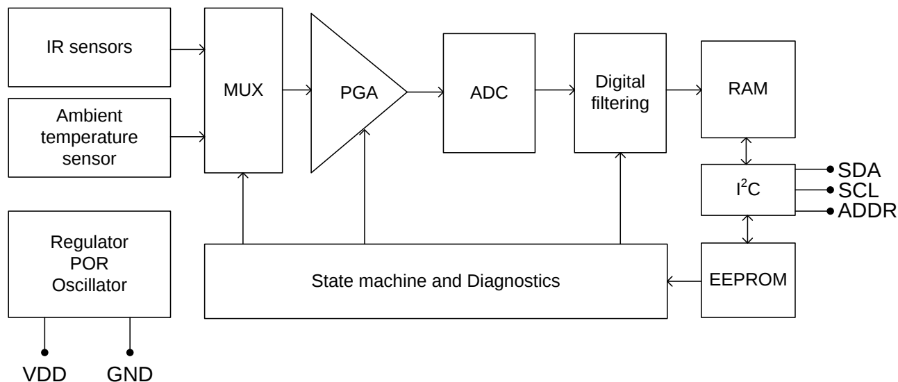
Figure 2 Block Diagram
