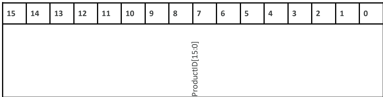
Figure 3 ID0
