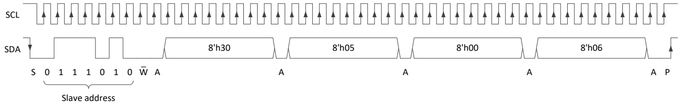
Figure 15 Addressed reset
