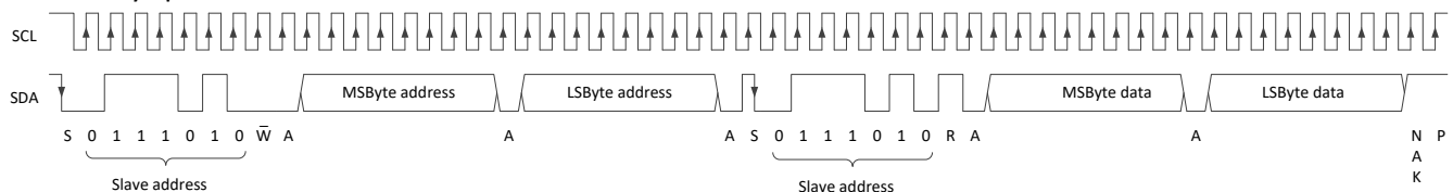
Figure 11 Addressed read
