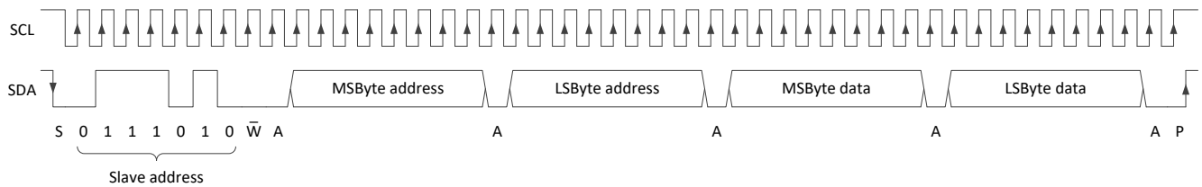
Figure 12 Addressed write
