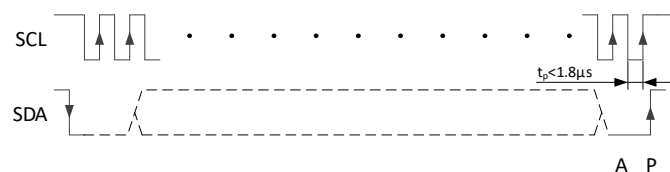
Figure 13 Reset command timing requirements
