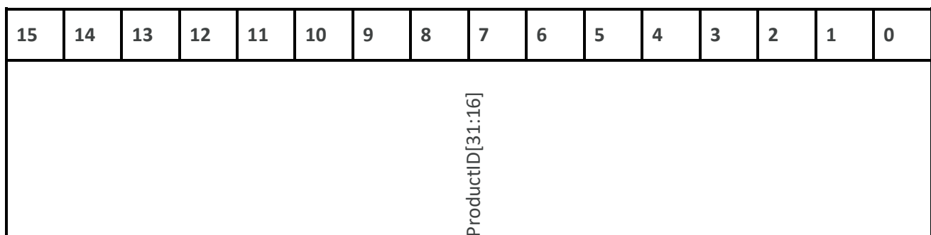
Figure 4 ID1
