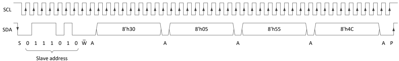
Figure 16 EEPROM unlock
