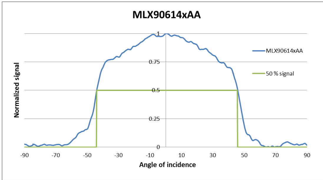
Figure 28 – Typical FOV of MLX90614xAA
