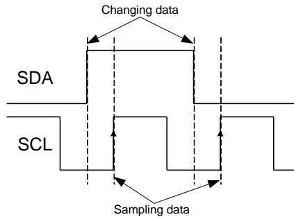
Figure 5 – Recommended timing on SMBus
