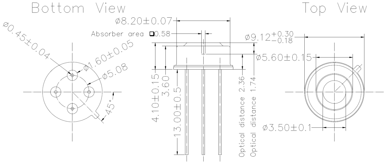
Figure 41 – Mechanical drawing of MLX90614xxA
