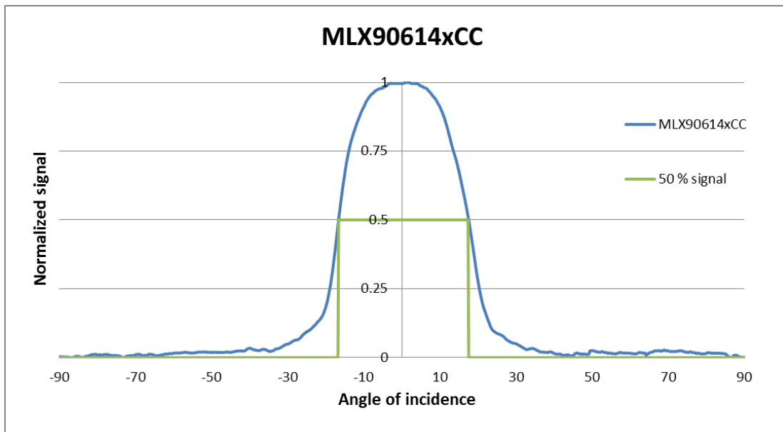
Figure 30 – Typical FOV of MLX90614xCC
