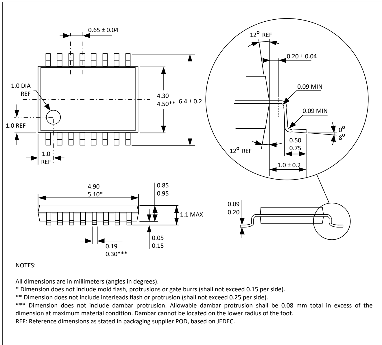
Figure 13 – TSSOP-16 Package Outline Dimensions
