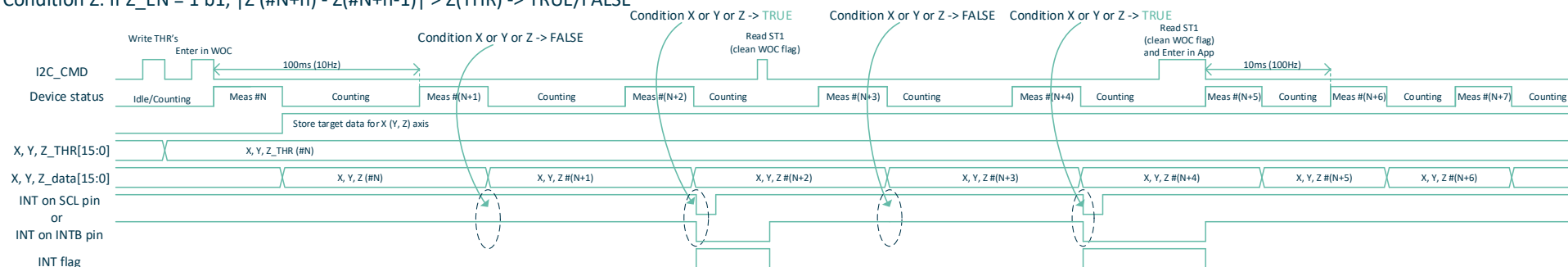
Figure 20 Dynamic Delta WOC example. Comparison of each measurement with the threshold after WOC enter, Single interrupt
