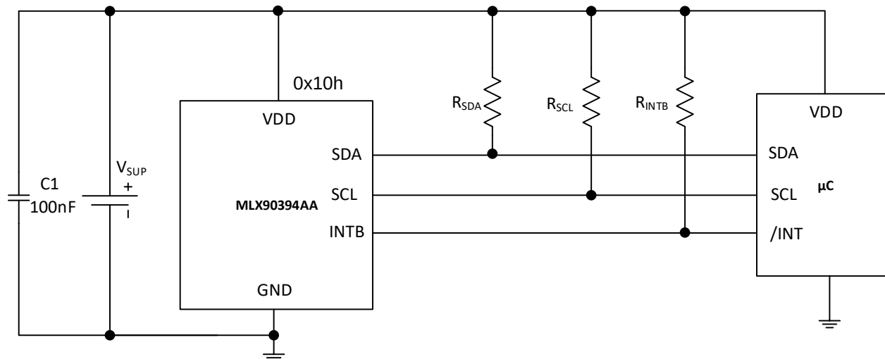
Figure 24: Recommended application diagram
