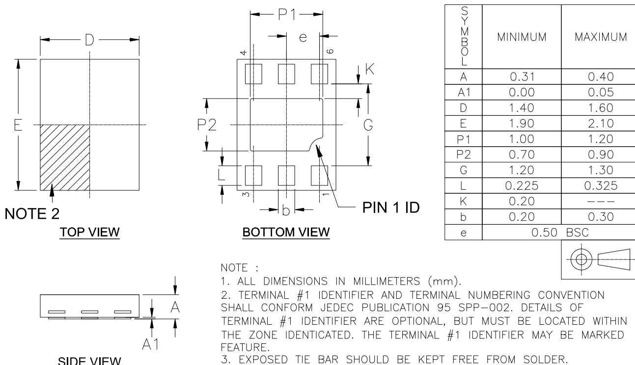
Figure 26 Preliminary Package Outline Drawing
