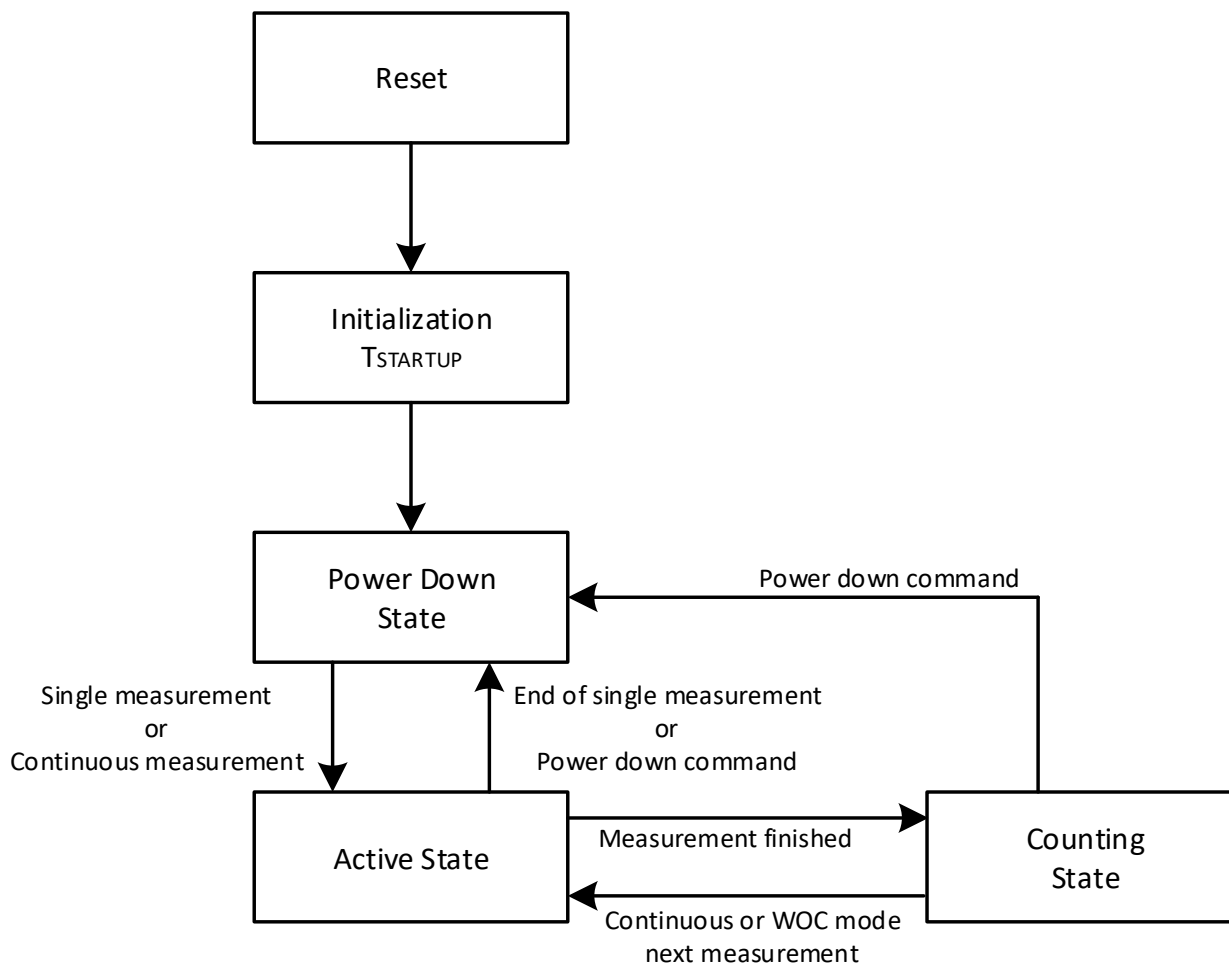
Figure 23: State Sequence flowchart
