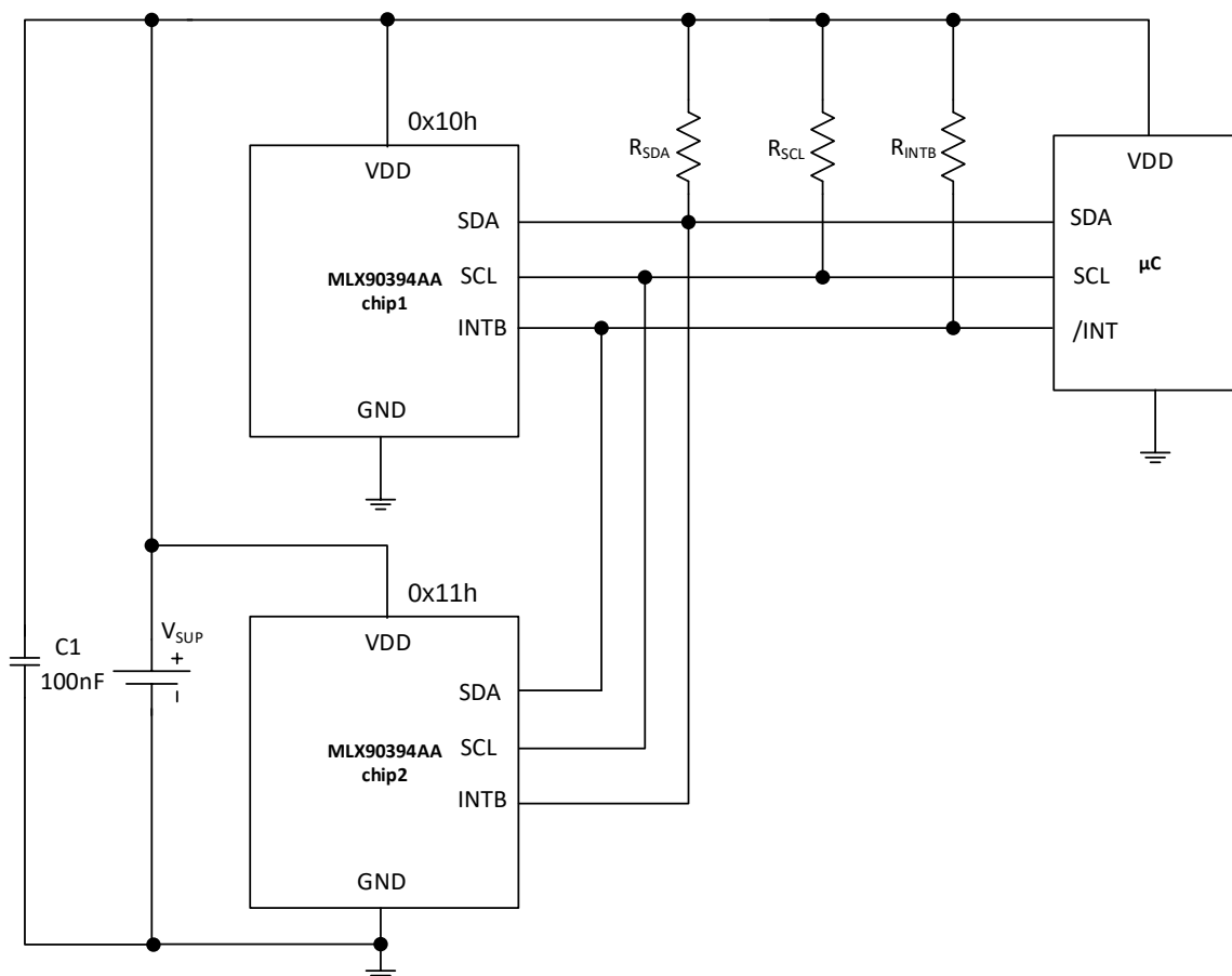
Figure 25 Application diagram with two MLX90394AA
