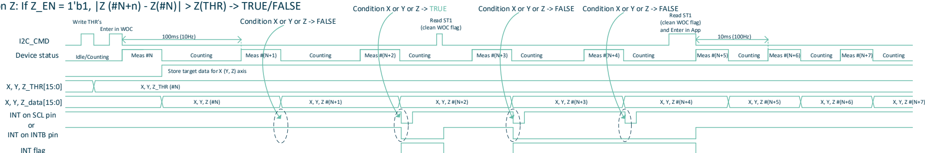
Figure 19 Static Delta WOC example with 1 st measurement after WOC enter. Repetitive interrupt
