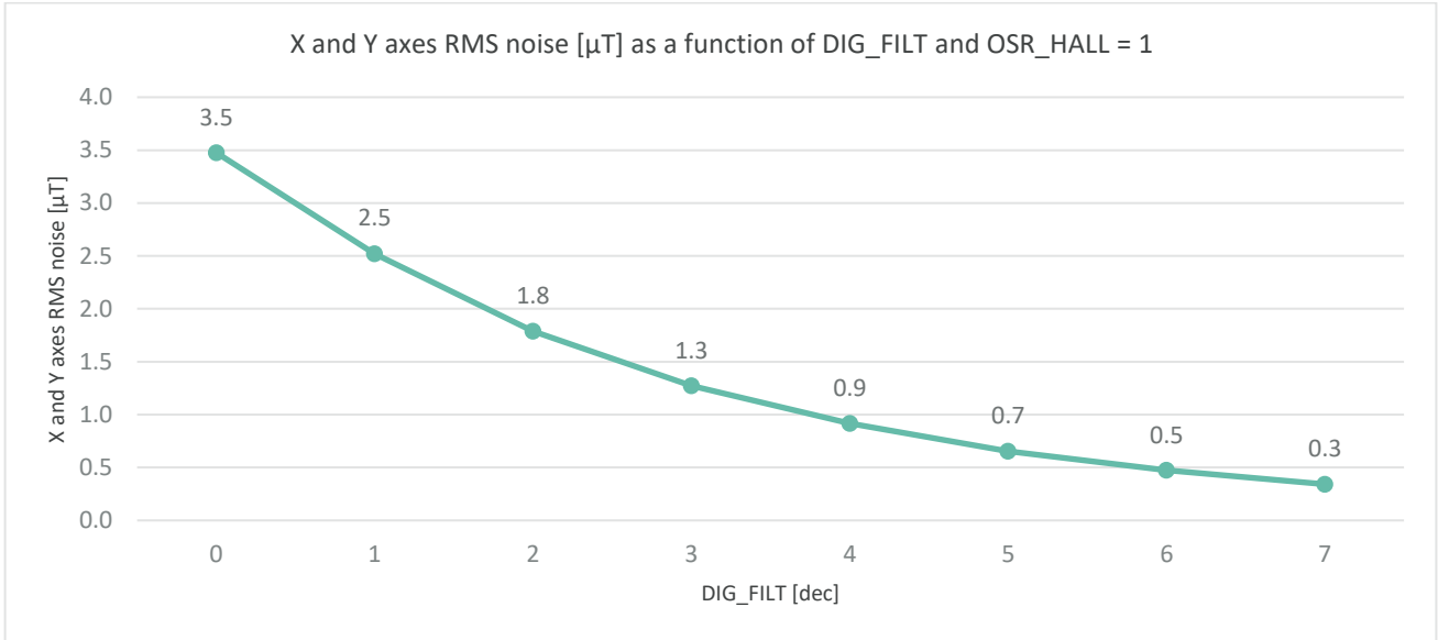
Figure 7 XY axes noise as a function of DIG_FILTER_HALL_XY. CONFIG=2
