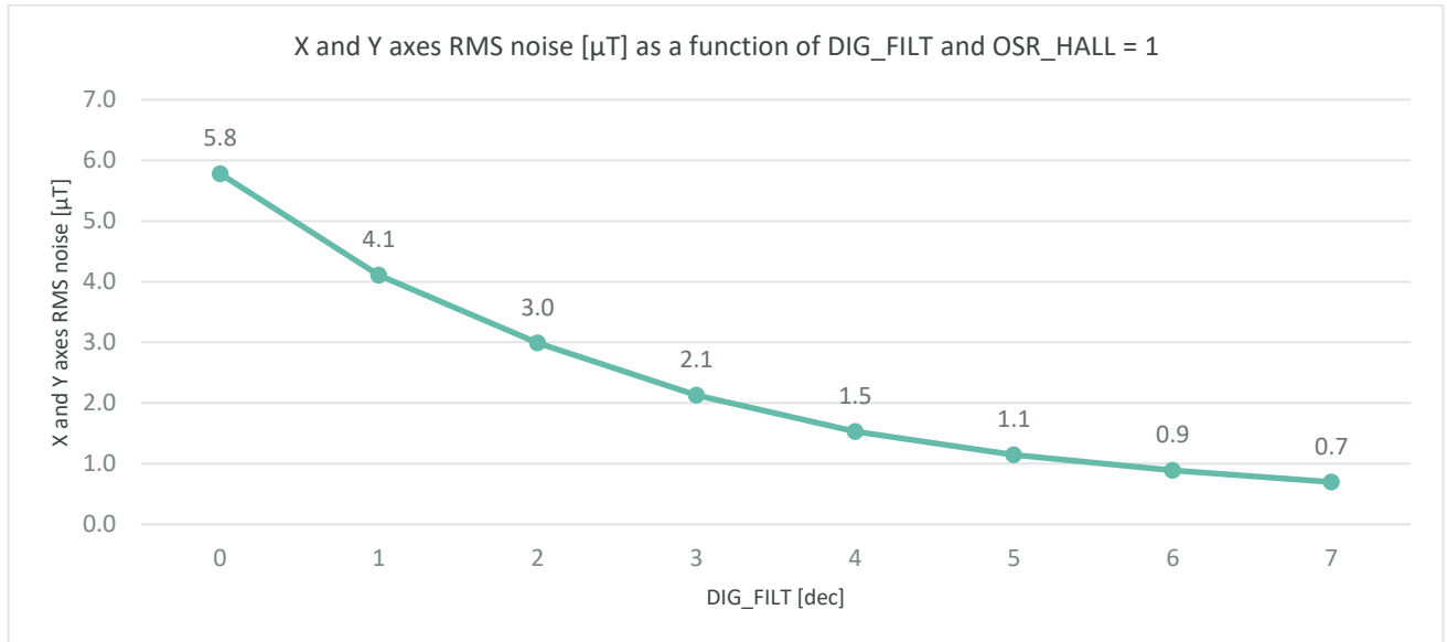
Figure 5 XY axes noise as a function of DIG_FILTER_HALL_XY. CONFIG=1
