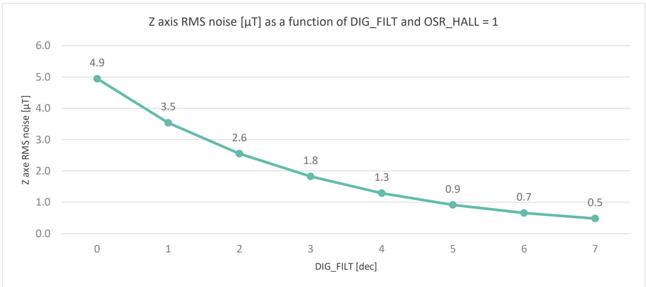
Figure 8 Z axis noise as a function of DIG_FILTER_HALL_Z. CONFIG=2
