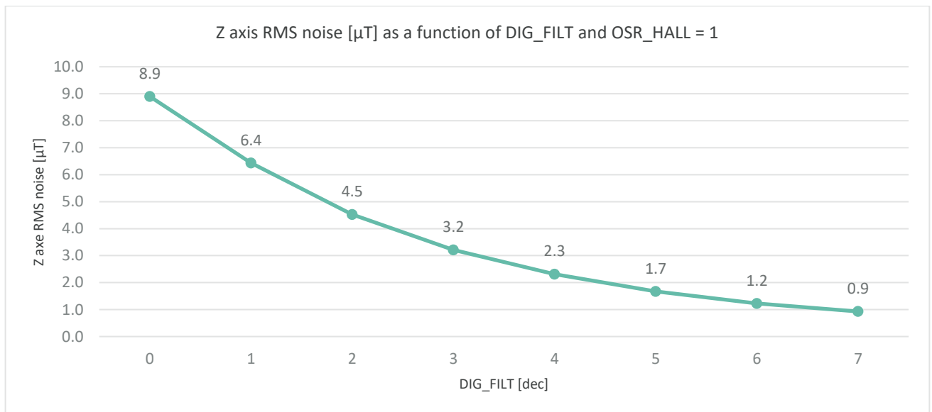
Figure 6 Z axis noise as a function of DIG_FILTER_HALL_Z. CONFIG=1
