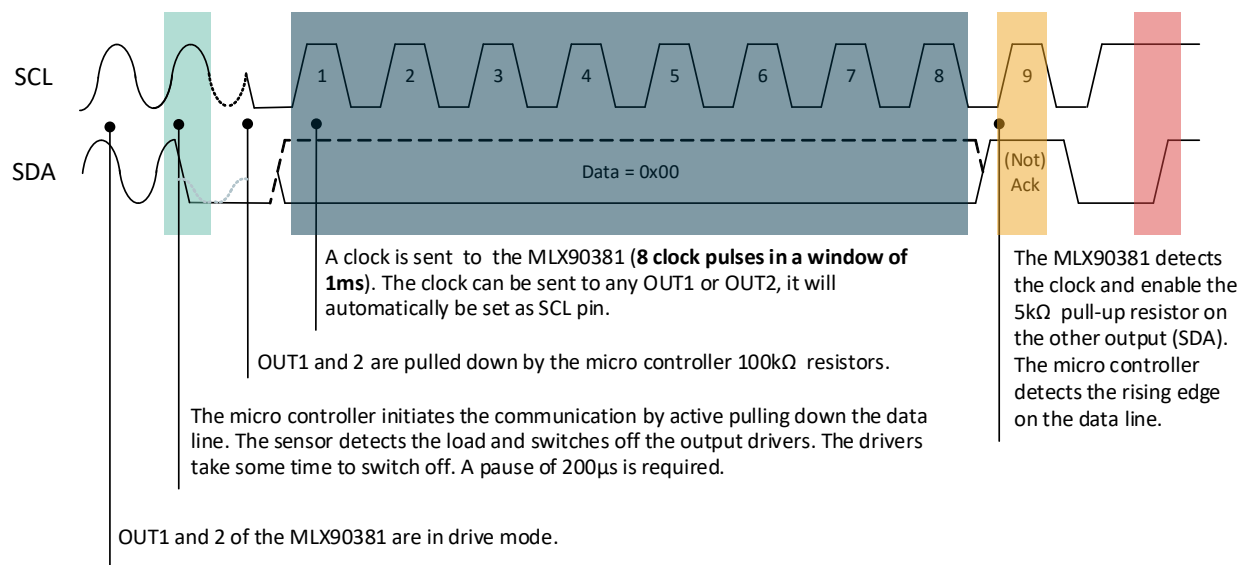
Figure 10 – Activation I 2 C interface
