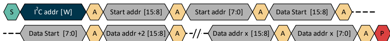
Figure 13 - Memory write register
