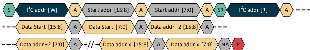
Figure 12 - Memory read MTP & register
