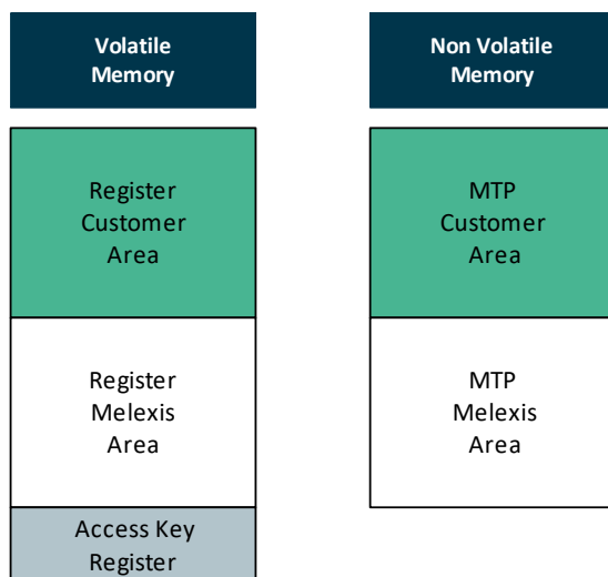
Figure 16 – Customer configuration register and MTP
