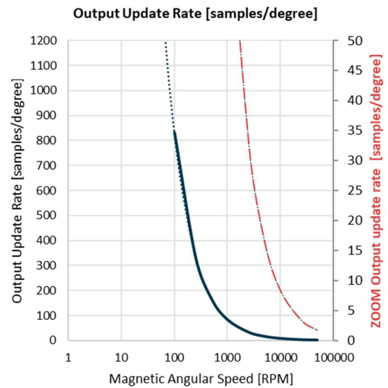
Figure 9 – Output update rate vs. magnetic angular speed
