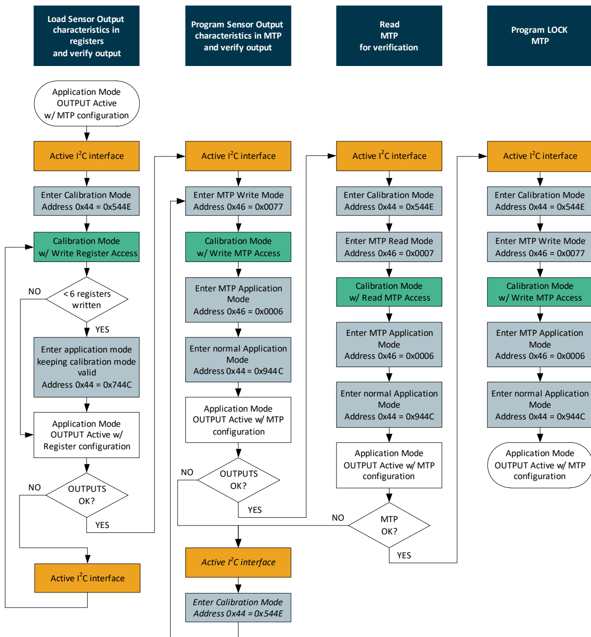
Figure 17 - Example flow for memory access key register
