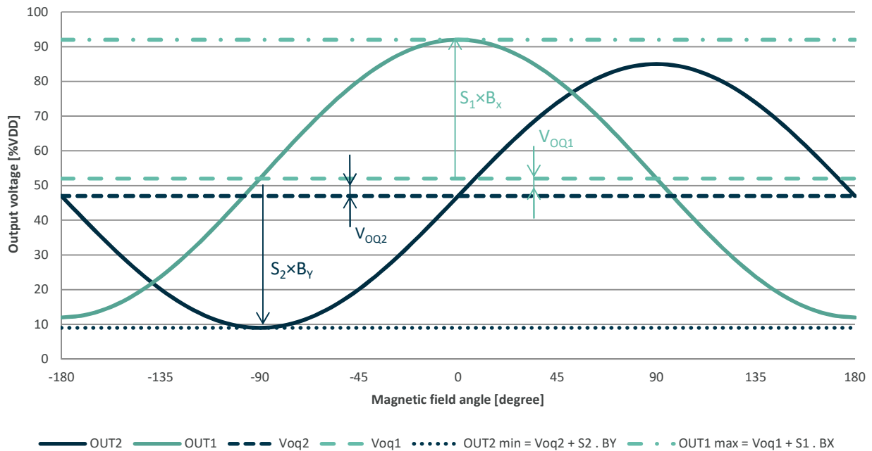
Figure 3 - Output characteristics
