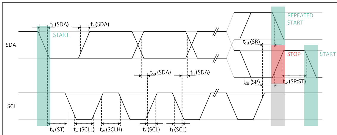
Figure 15 – I 2 C timing diagram
