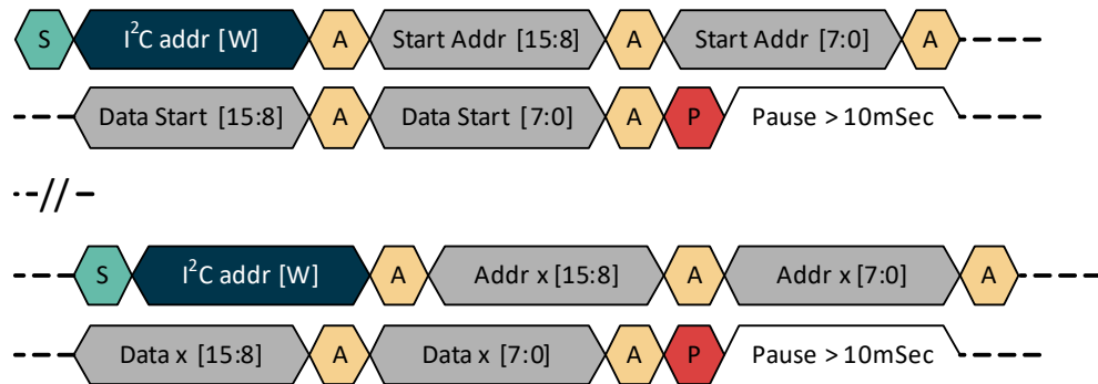
Figure 14 - Memory write MTP
