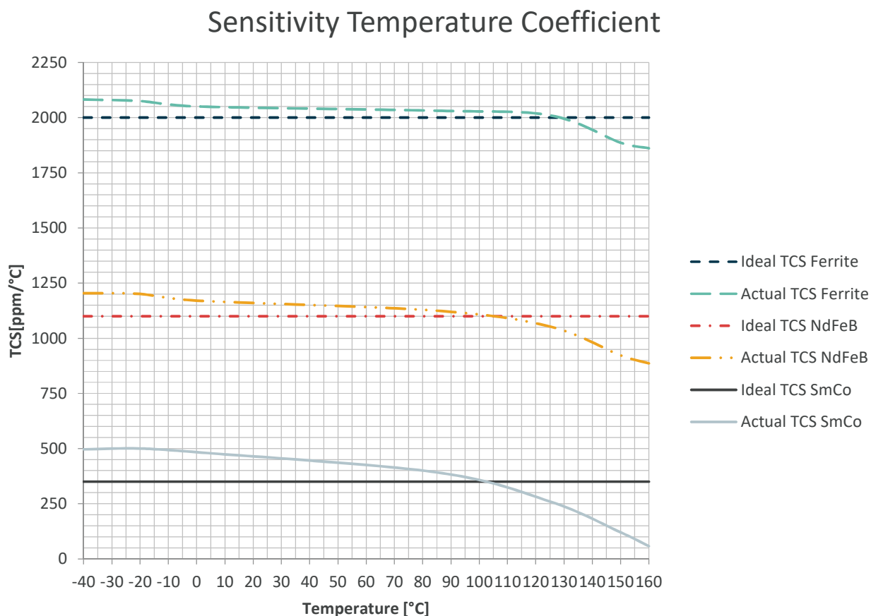
Figure 6 – Target TCS vs. 2 nd order TCS (3V3)
