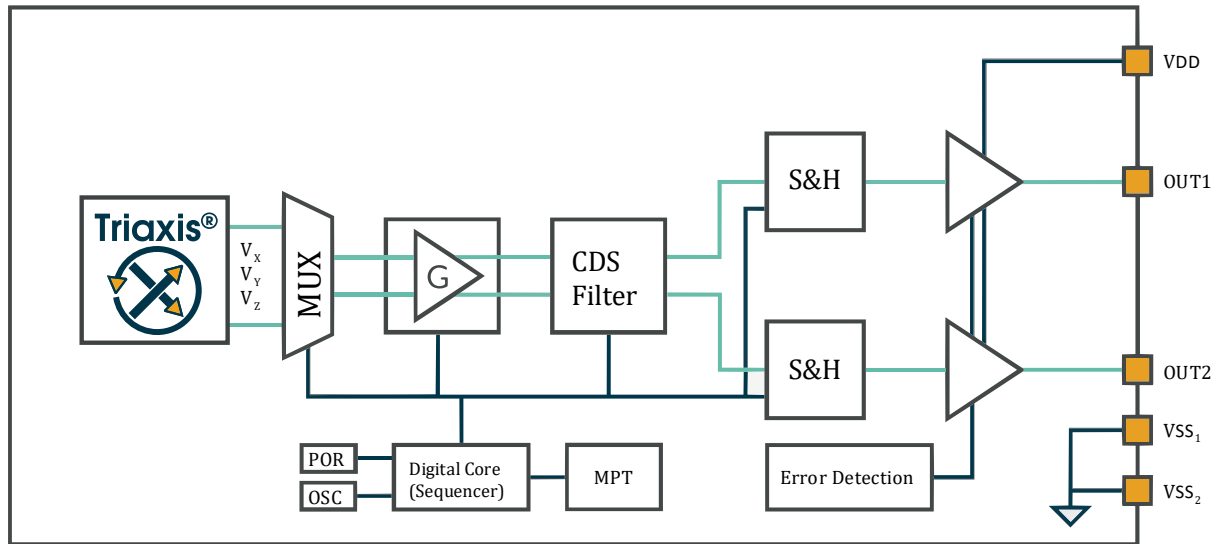
Figure 1 – Functional diagram
