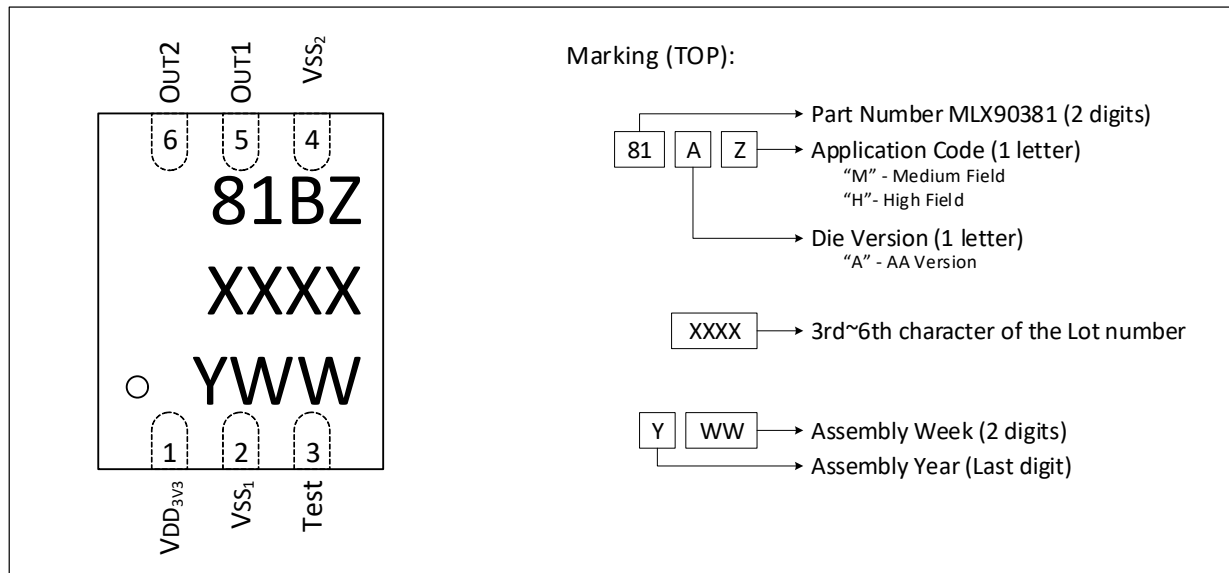
Figure 23 – DFN-6 pin out and marking 5V
