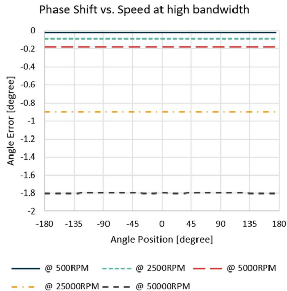
Figure 8 - Signal phase shift vs. magnetic angular speed
