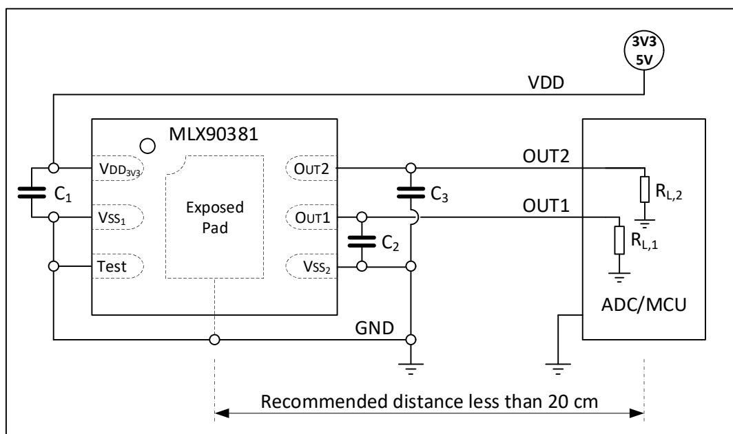
Figure 19 – Recommended application diagram
