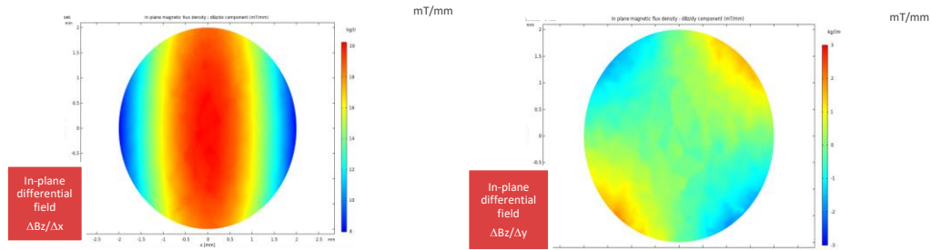
Figure 3 – Magnetic axial- field differential fields ( \Delta B_z/\Delta X ), ( \Delta B_z/\Delta Y ) for the fig. 2
