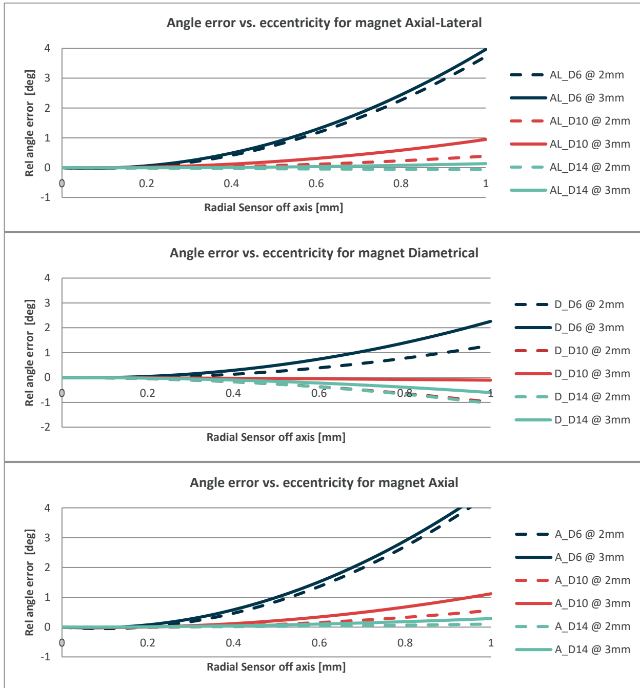
Figure 11 : max. Non-linearity error vs. radial sensor off axis & Axial distance from Magnet to Sensor
