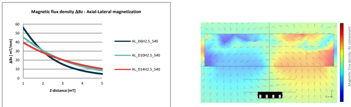
Figure 7 : Magnetic flux density \Delta B_z & flux lines for an axial-lateral magnetized magnet
